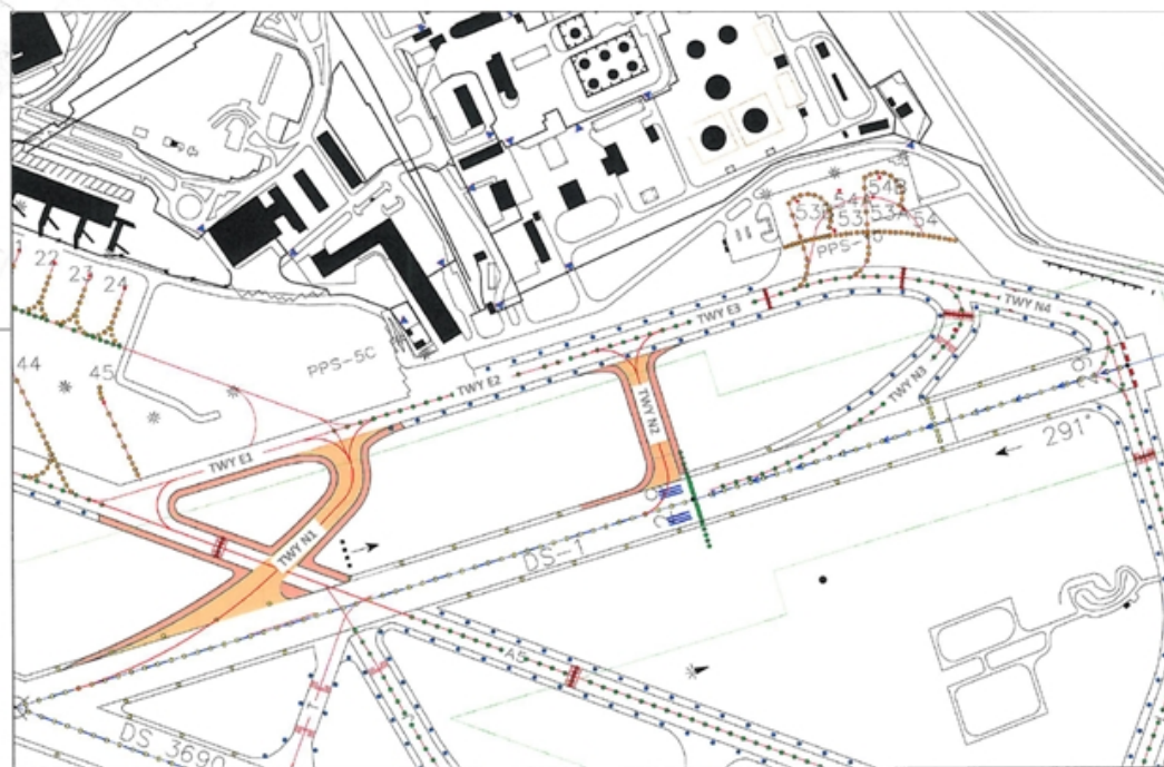
new taxiways
